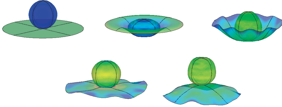
Figure 4.2: AVI methodology: collision between an elastic sphere and a plate (Cirak and West [2004]).
