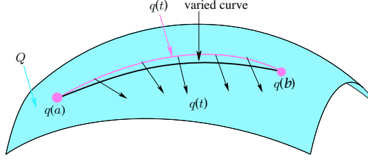
Figure 1.1: The configuration space form of Hamilton's principle
