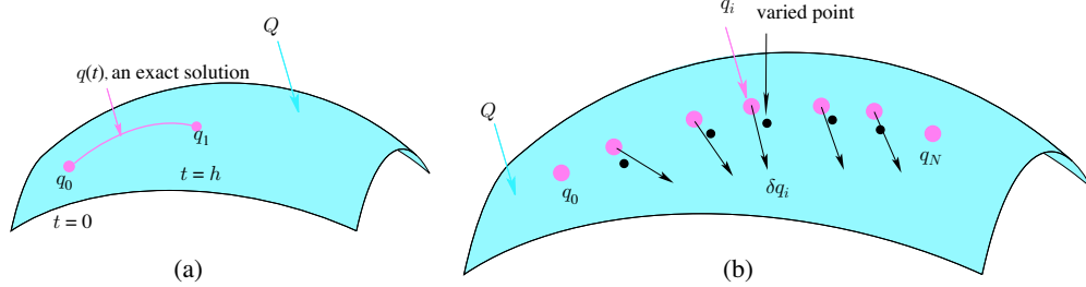
Figure 1.2: The discrete form of the configuration form of Hamilton's principle
