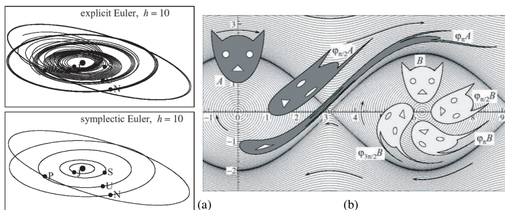
Figure 2.1: (a) Variational integrators give good qualitative behavior for comparable computational effort. (b) Variational integrators preserve the symplectic form in phase space (area in two dimensions). These figures are due to Hairer, Lubich, and Wanner [2001], to which we refer for further information.
