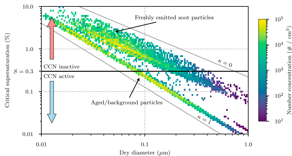
Figure 16. Two-dimensional number distribution as a function of particle dry diameter and critical supersaturation. The black horizontal line indicates a given environmental supersaturation threshold (here 0.3% as an example). Based on this the particles can be categorized as cloud condensation nuclei (CCN) inactive and CCN active.
