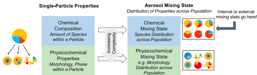
Figure 3. Illustration of our terminology. We separate the properties that describe single particles (section 2.1) from the distribution of these properties across the population (section 2.2). It is further useful to separate the aspects that pertain to chemical composition and its distribution across the population from the aspects that include not only chemical composition but also morphology and phase, which together constitute the physicochemical properties for individual particles and the physicochemical mixing state of the population.
